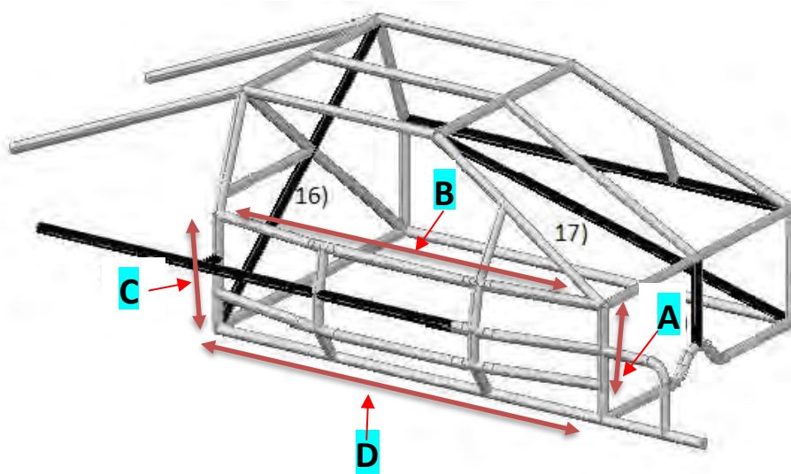
Anti-spear plate Diagram
