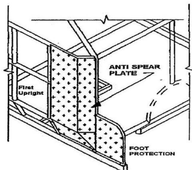
Anti-Spear Plate / Foot Protection diagram
