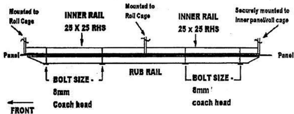
Rub Rail Diagram
