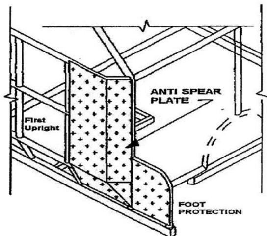
Anti-Spear Plate / Foot Protection diagram
